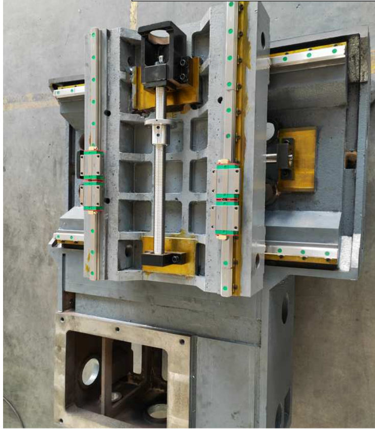
HIWIN Linear guideway for all X,Y,U,V,Z, wire drum and wire tension.
