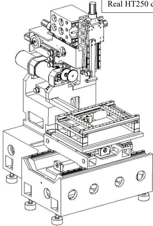
High rigidity "C" structure
