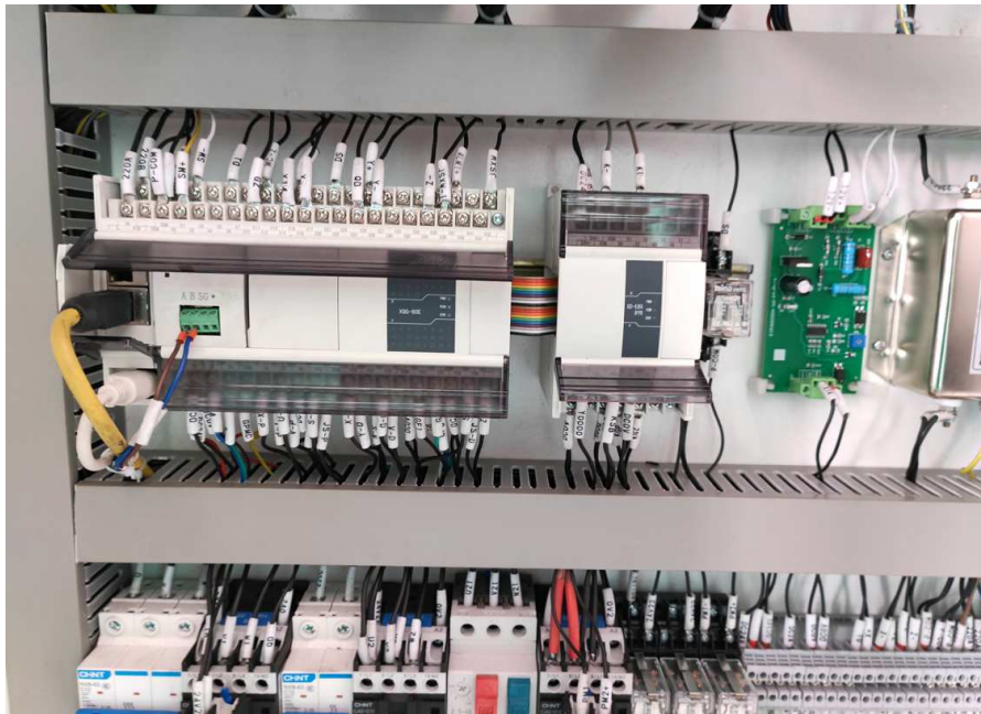
KCUT PLC control, communication with Internet protocol, super-fast speed, and good anti-interference capacity.
